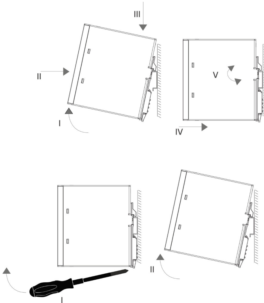
Figure 6: Assembly
