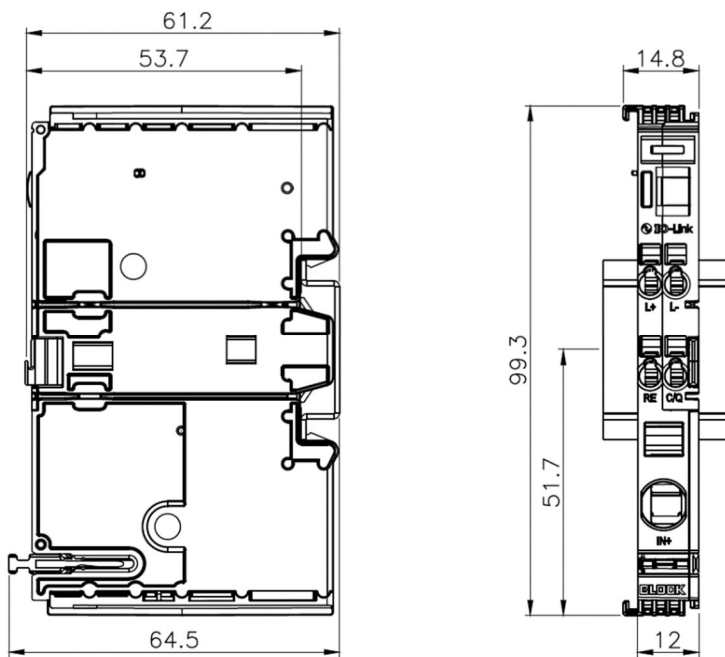
Figure 2: Dimensioning IO-LINK
